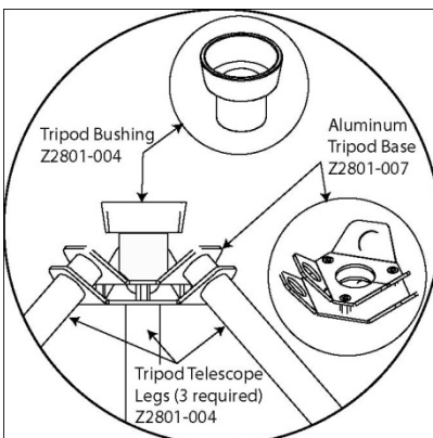
Fig. 10. Tripod Assembly
