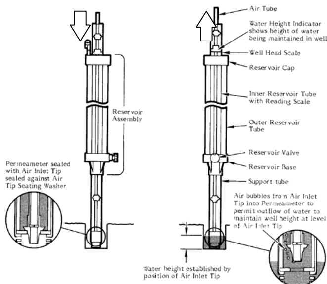
Fig. 12. Illustration of Air Inlet status.
