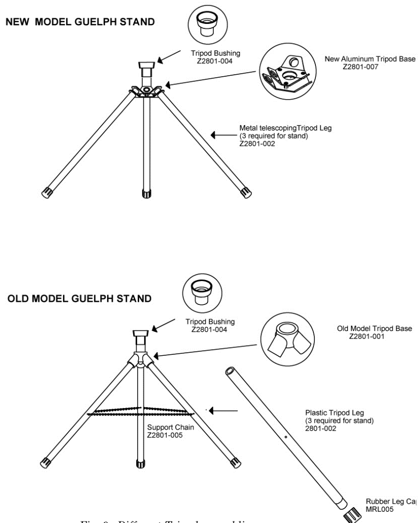
Fig. 9. Different Tripod assemblies
