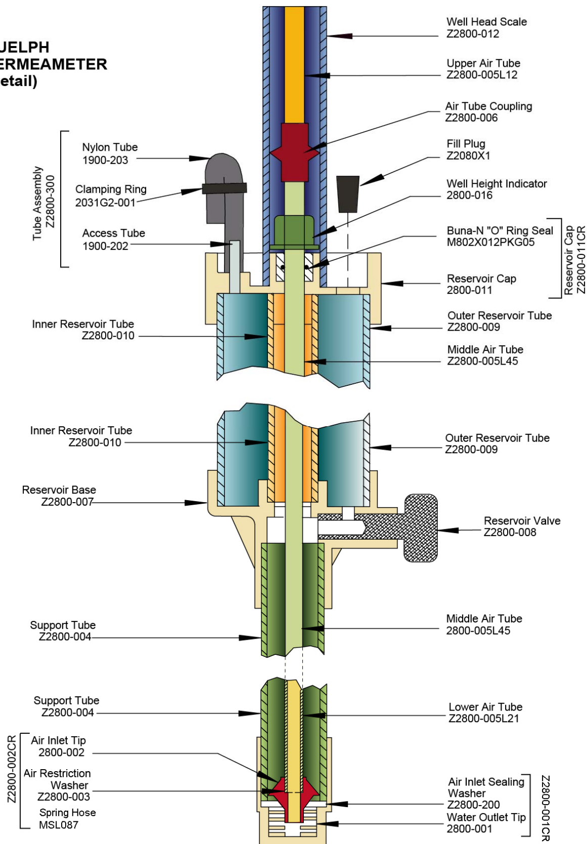
Fig. 50- Guelph Components.
